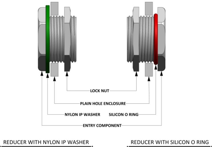
ARRANGEMENT OF REDUCER IN PLAIN ENTRIES
