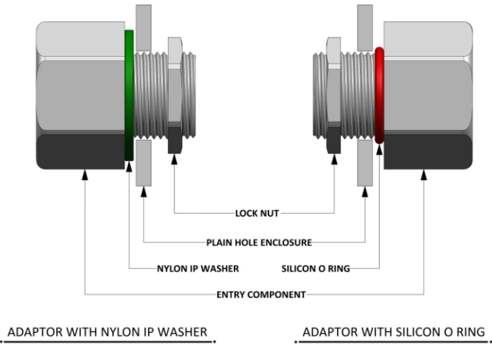
ARRANGEMENT OF ADAPTOR IN PLAIN ENTRIES
